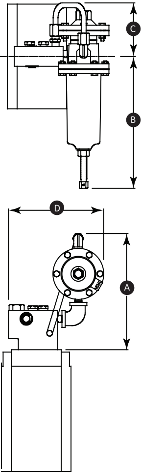
ZSC 320 - 100 Control Loop
